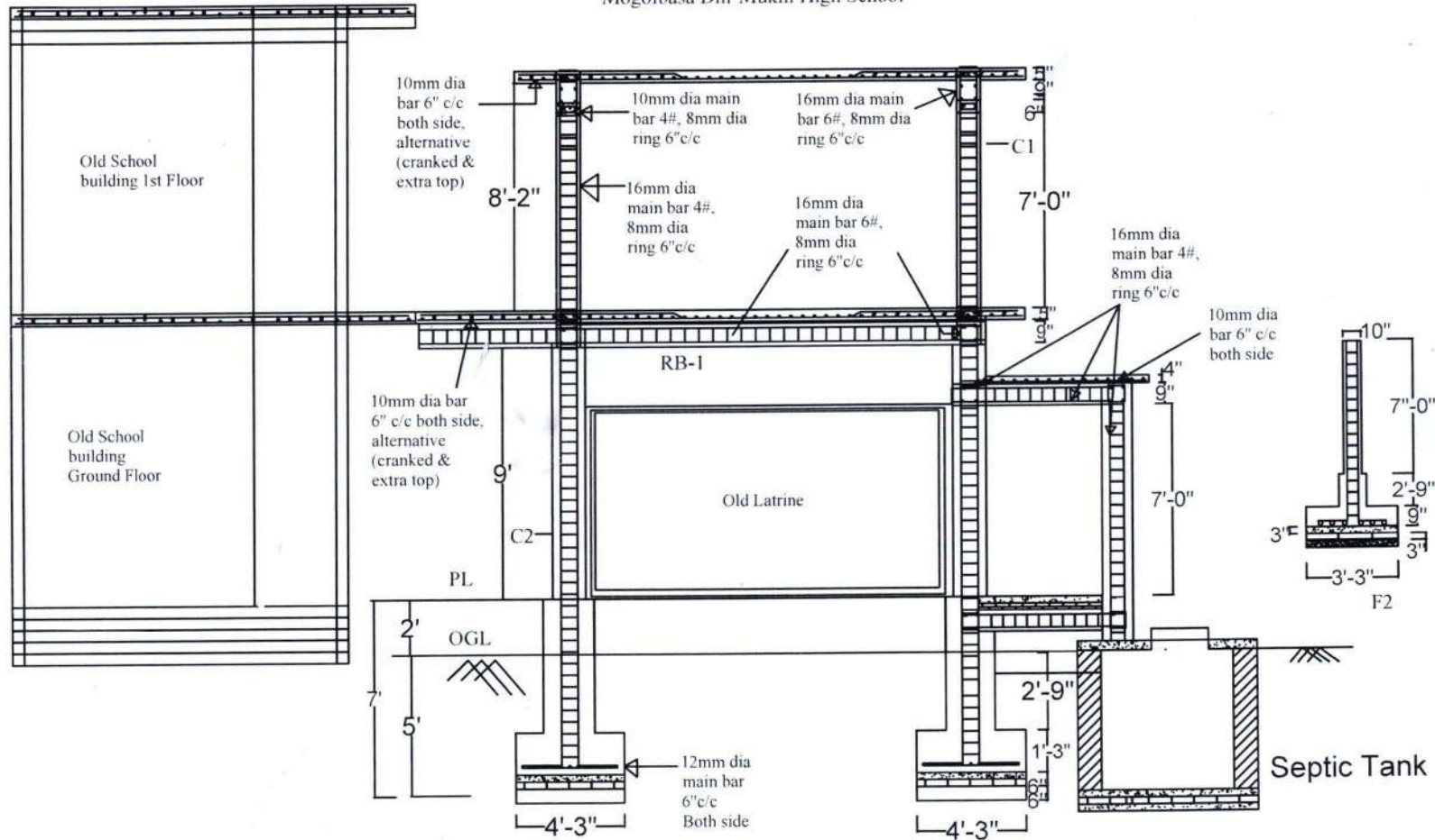
X- Section
