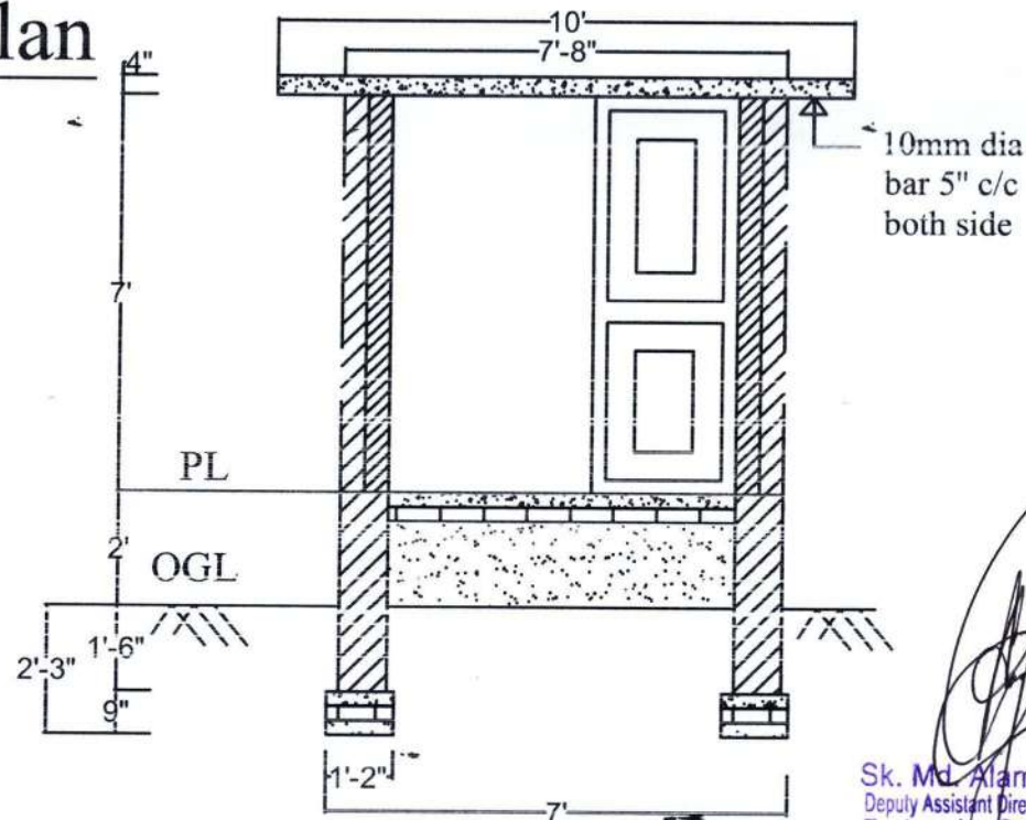
Toilet X-Section
