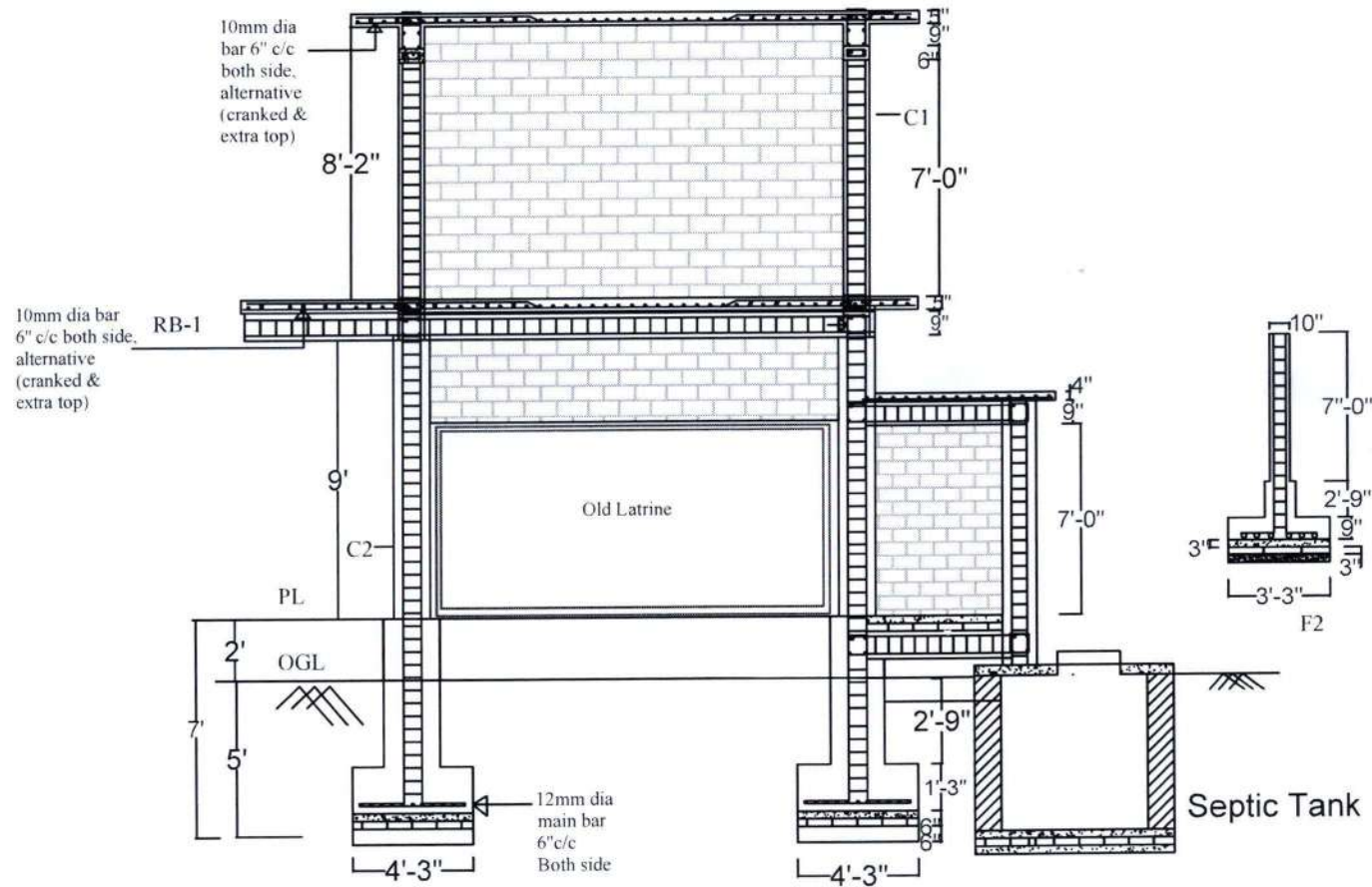
X- Section
