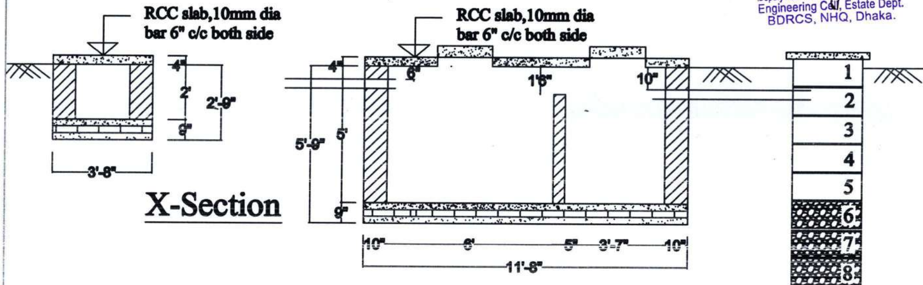
X- Section Inspection Chamber, Septic tank & Sock well
