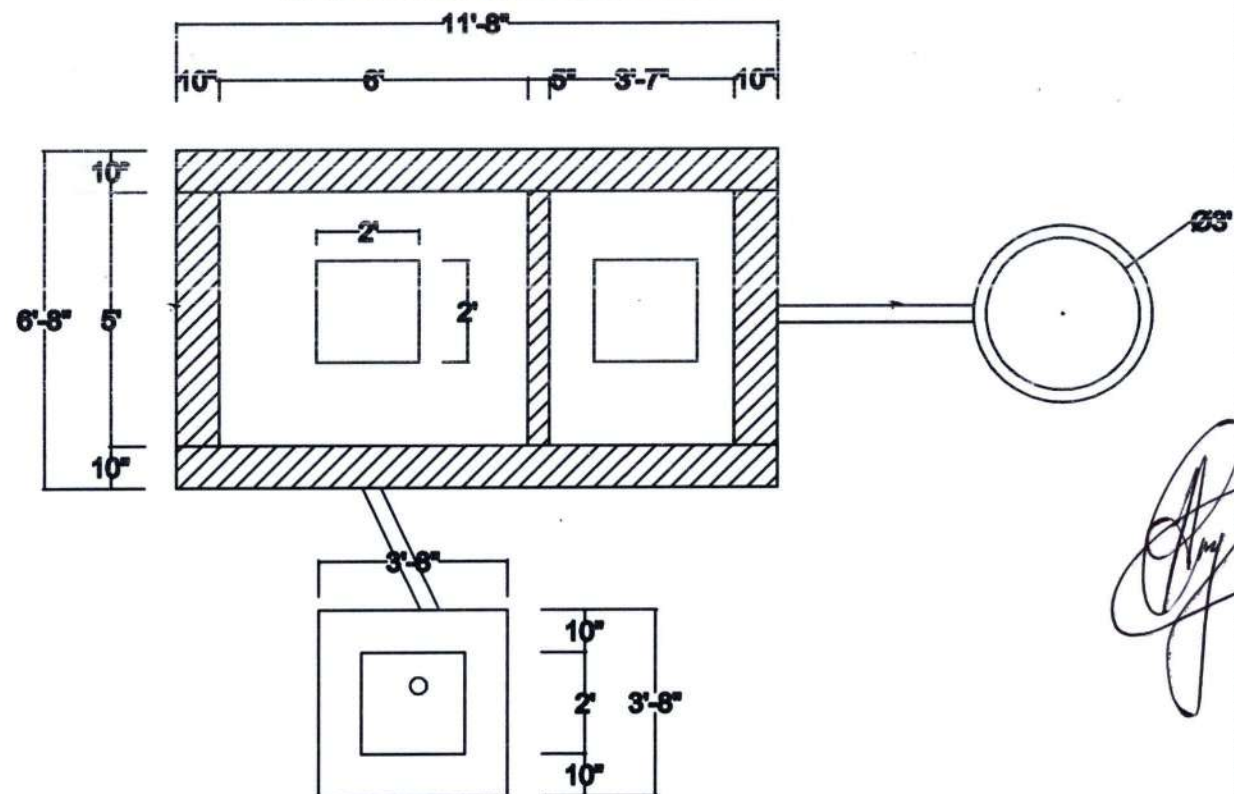
Septic Tank, Inspection Chamber & Sock Well
