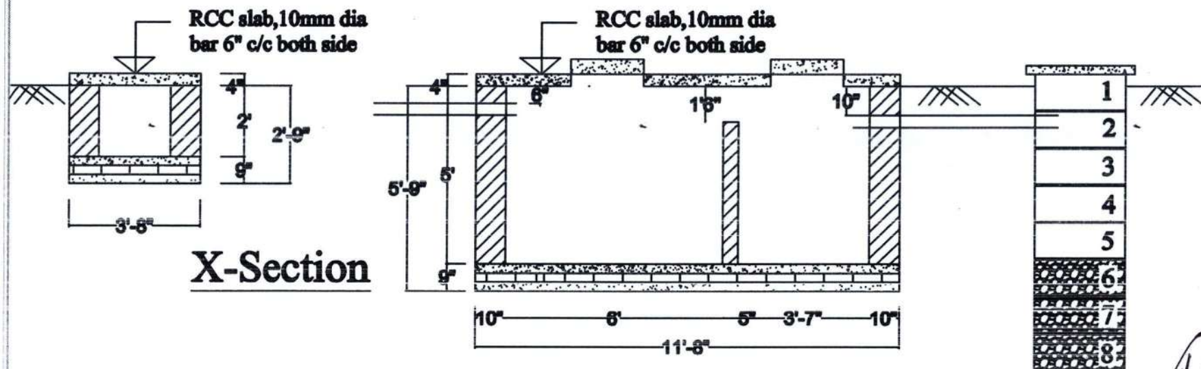
X- Section Inspection Chamber, Septic tank & Sock well
