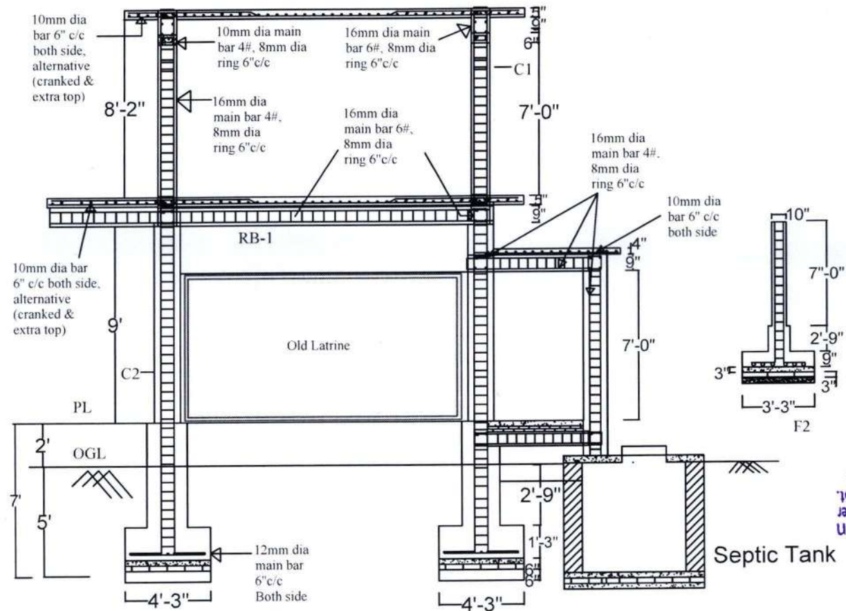
X- Section
