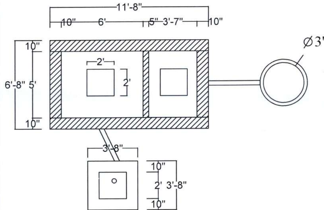
Septic Tank, Inspection Chamber & Sock Well
